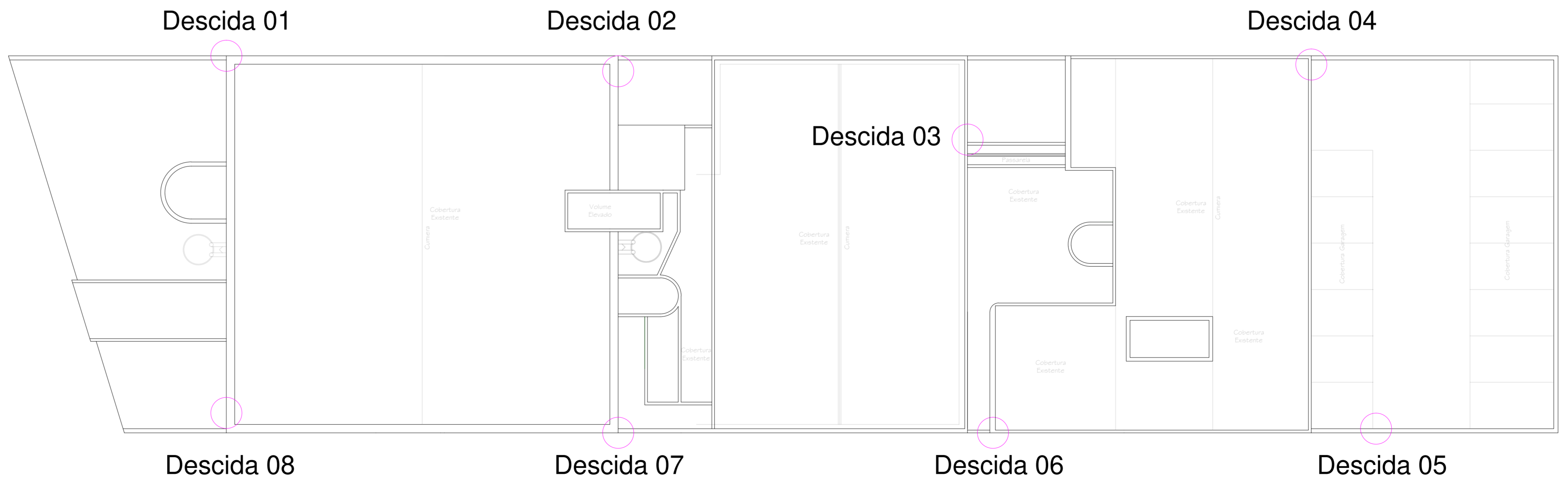
LOCALS DAS DESCIDAS escala 1/150
